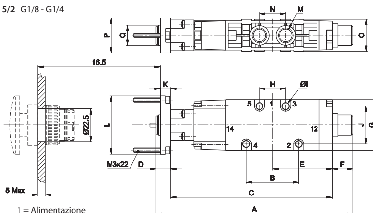
5/2 G1/8 - G1/4
