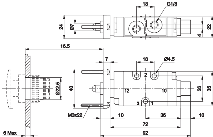
3/2 NC-NO G1/8
