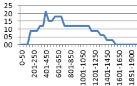
“Automatic Delayed Command” 2 simultaneous clamps 130mS delay
