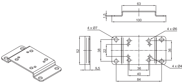
HZRE30300 Horizontal bracket
