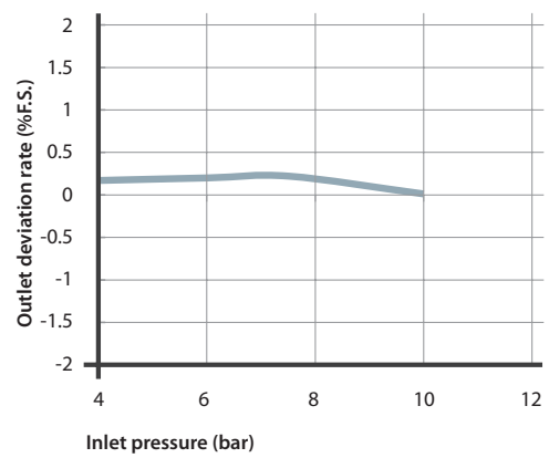
Pressure characteristic
