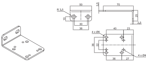
HZRE30310 Wall bracket
